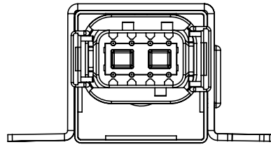
Connector view with mounting bracket
